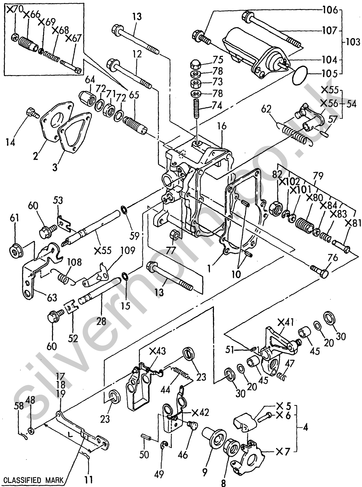
Fig. 12 GOVERNOR
