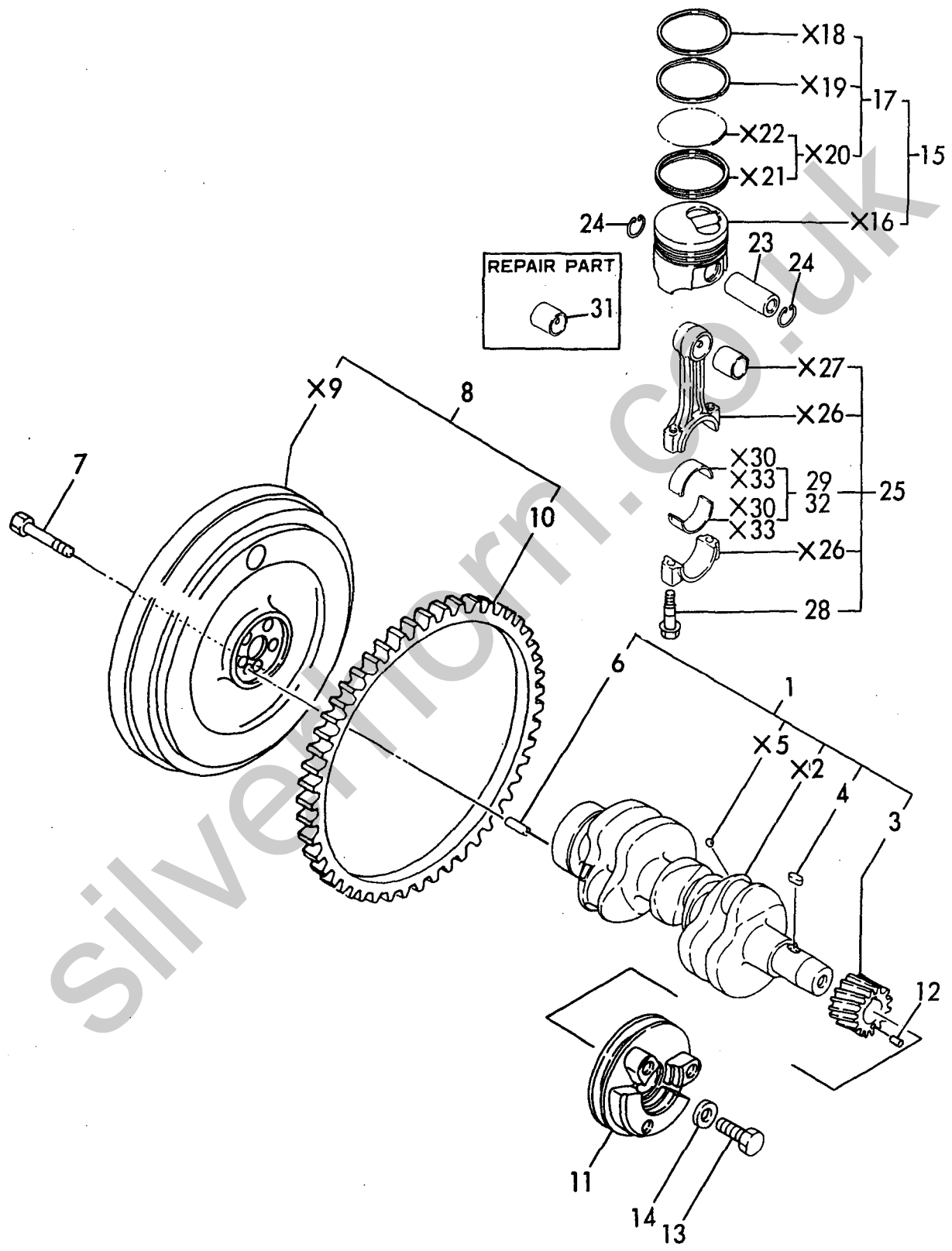
Fig. 7 CRANKSHAFT & PISTON
