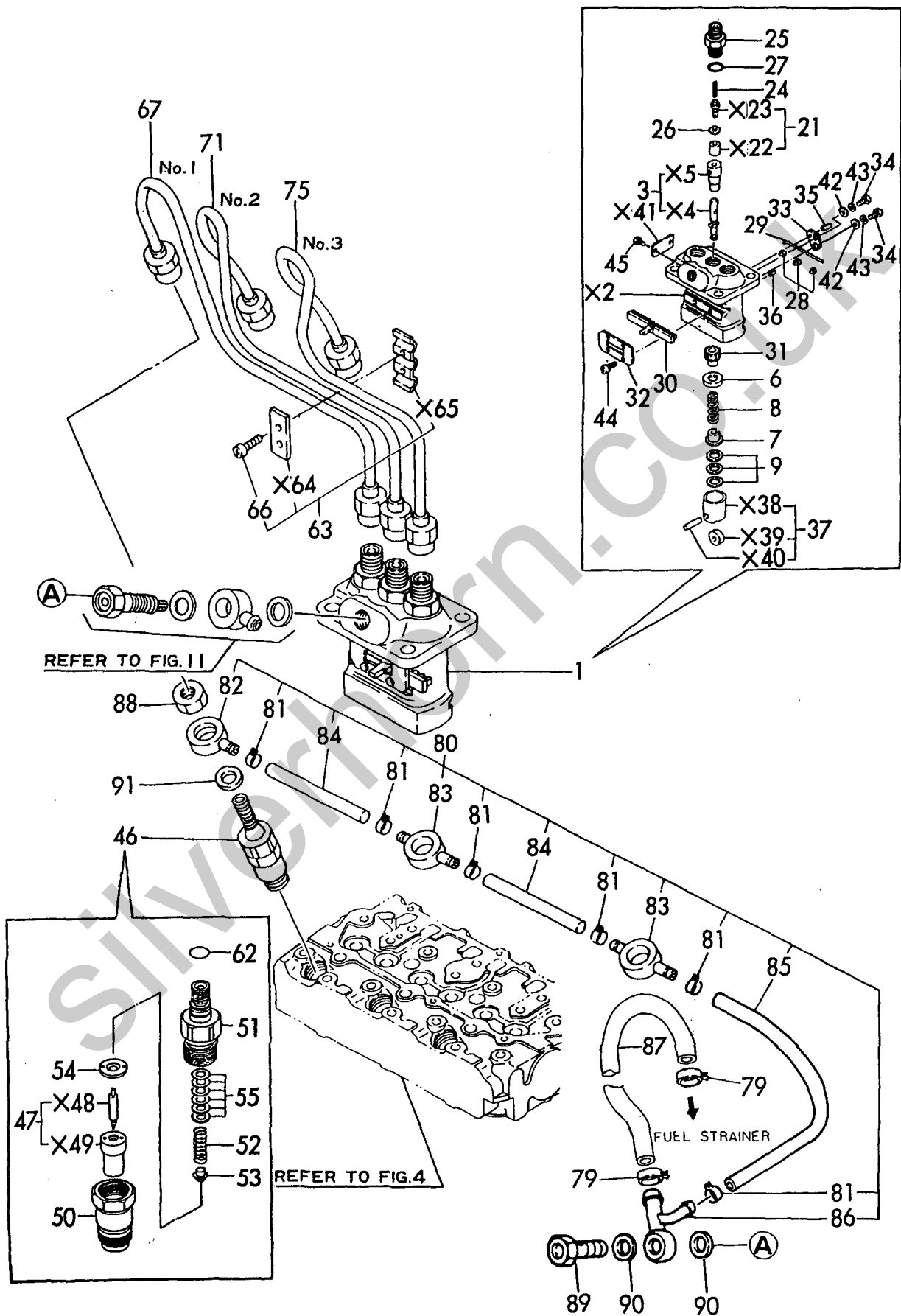
Fig. 10 FUEL INJECTION DEVICE
