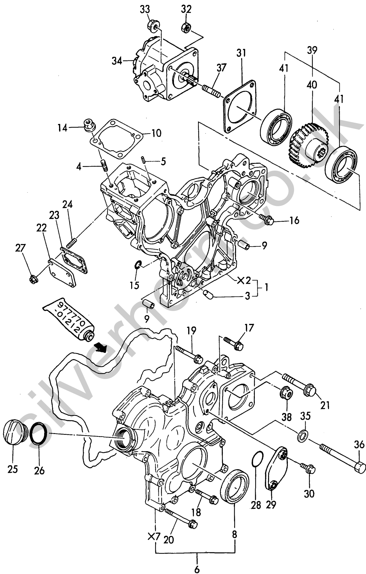
Fig. 2 GEAR HOUSING
