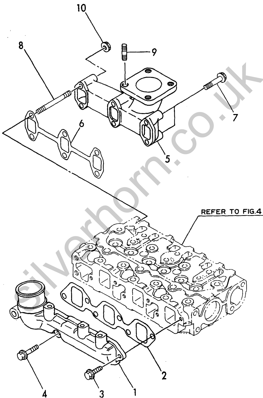
Fig. 5 SUCTION & EXHAUST MANIFOLD
