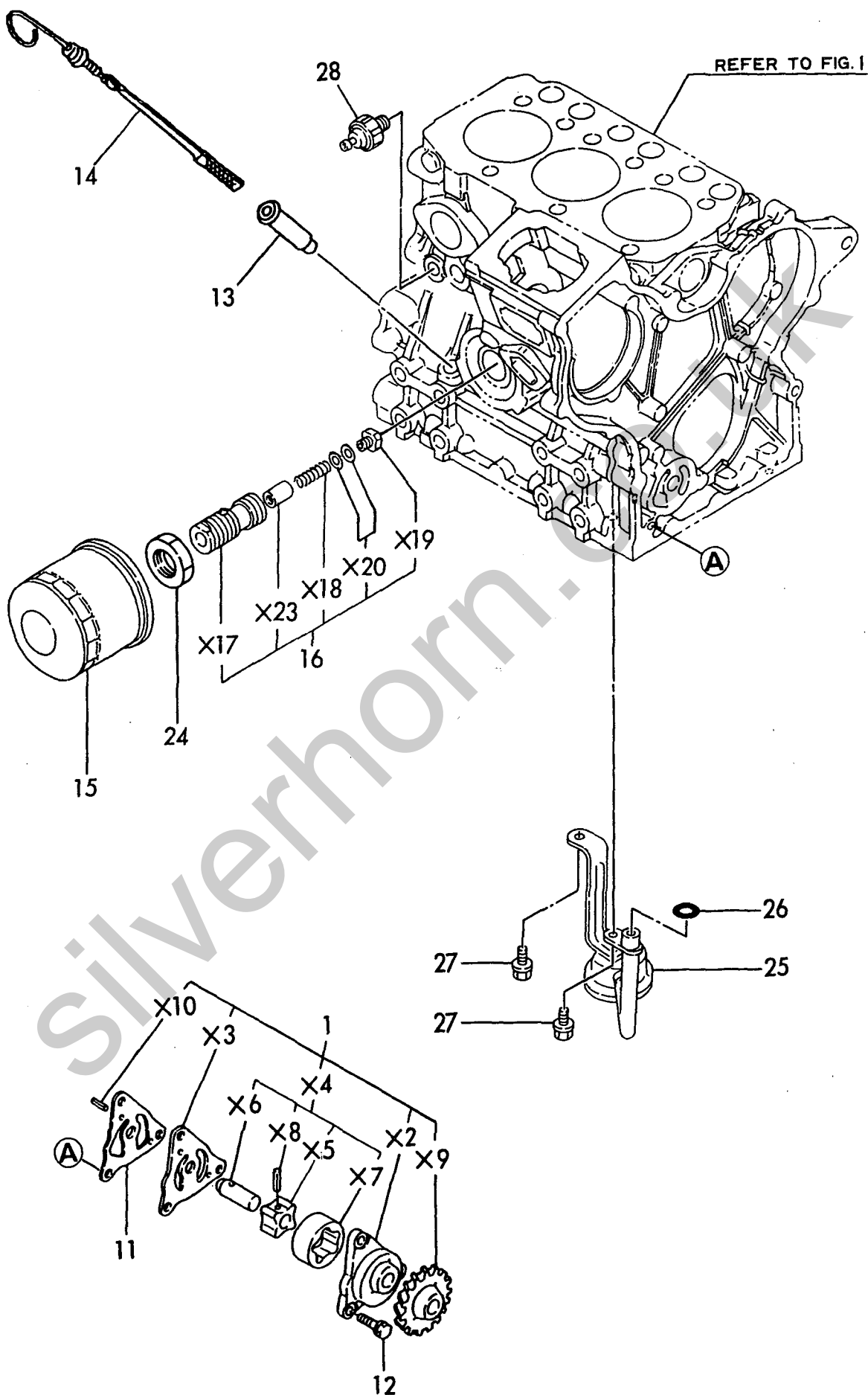
Fig. 8 LUB. OIL SYSTEM
