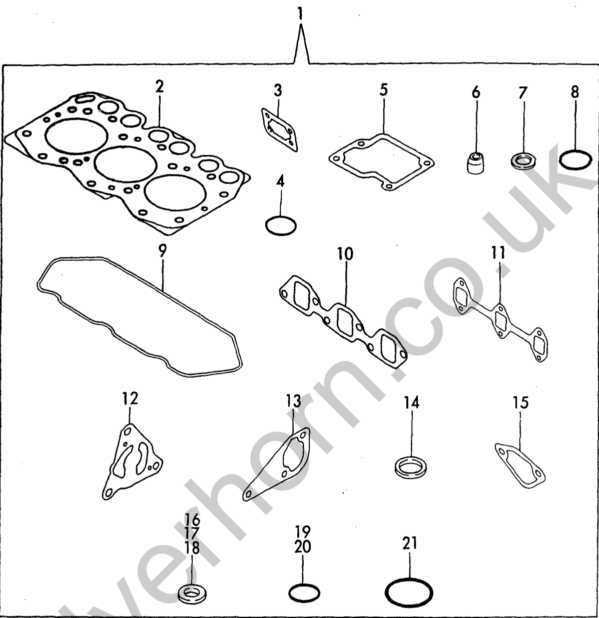
Fig. 15 GASKET SET & TOOL (OPTIONAL)
