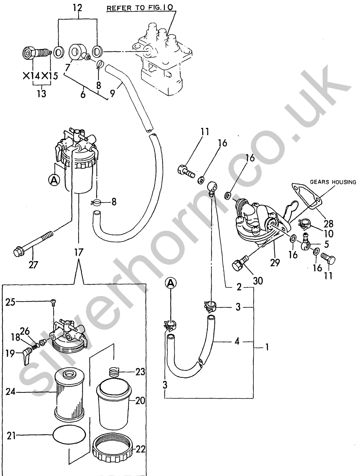
Fig. 11 FUEL LINE
