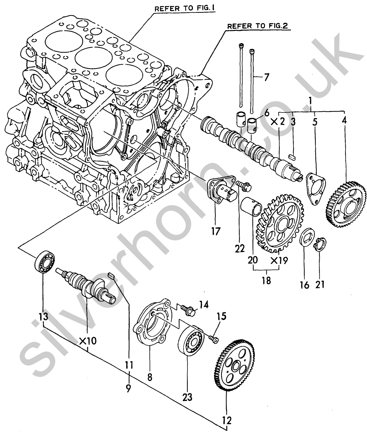
Fig. 6 CAMSHAFT & DRIVING GEAR
