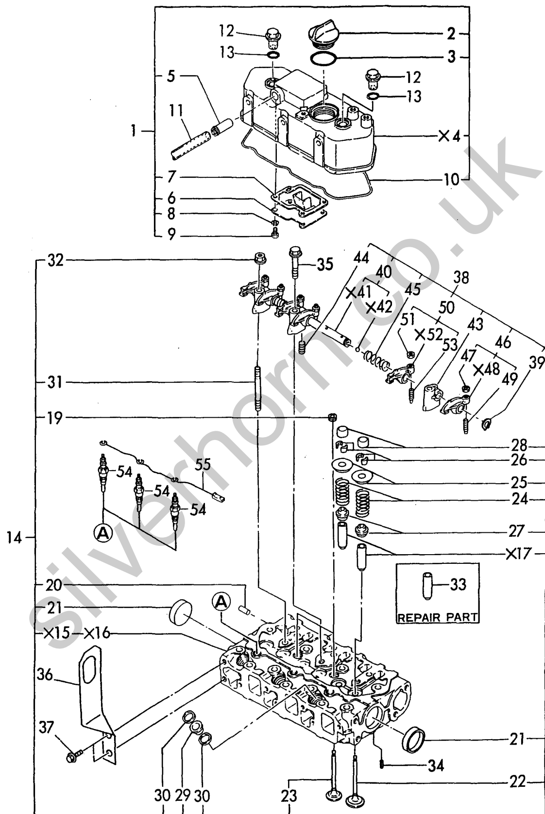
Fig. 4 CYLINDER HEAD & BONNET
